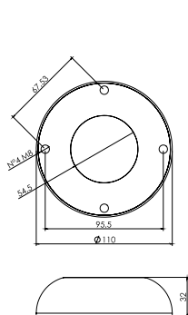
FIXED JOINT SGF 110
