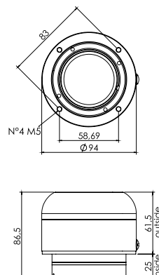
SWIVEL JOINT HYGIENIC DESIGN GG21 94 Hanging-unit-side joint Diameter 94 mm Resistant to load up to 30 kg IP66 - IP69K as standard
