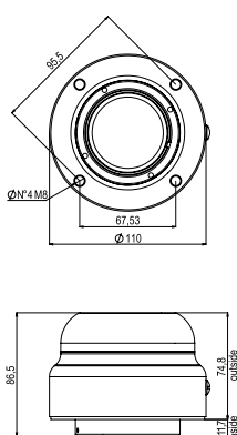
SWIVEL JOINT HYGIENIC DESIGN GG21 110 Machinery-side joint Diameter 110 mm Resistant to load up to 30 kg IP66 - IP69K as standard
